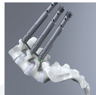
Multi-Level Capabilities
