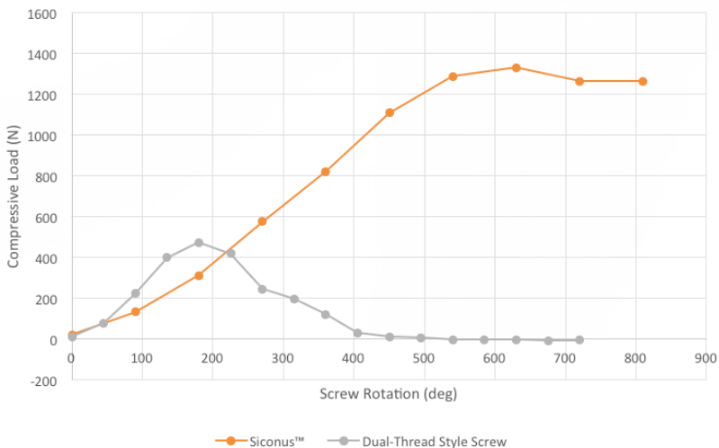
Screw Compression Comparison
